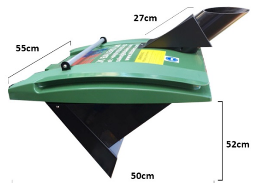
Glass Crusher Dimensions
